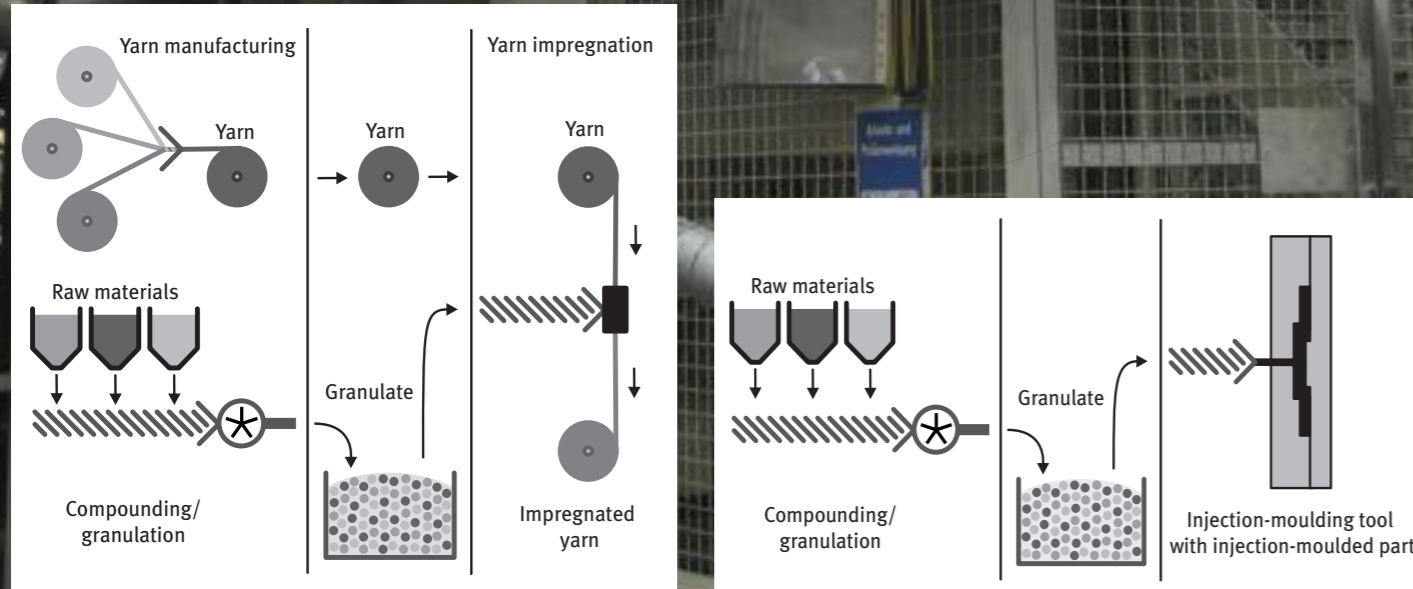
Schematic illustration of production of LMF: Solvent-free yarn impregnation protects resources.
